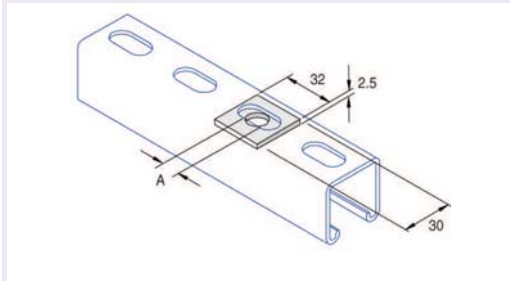
Internal Square Plate Washers
