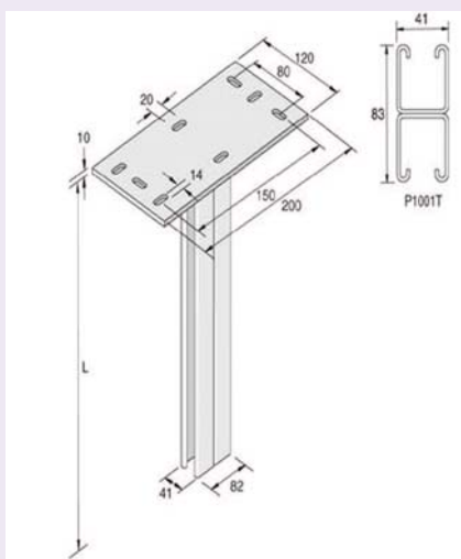
Double Channel 41X41
