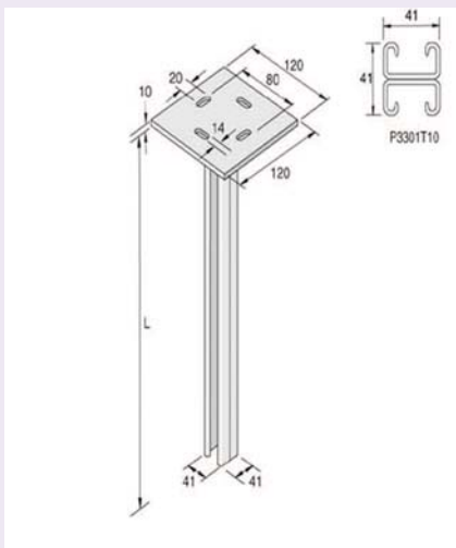
Double Channel 41X21
