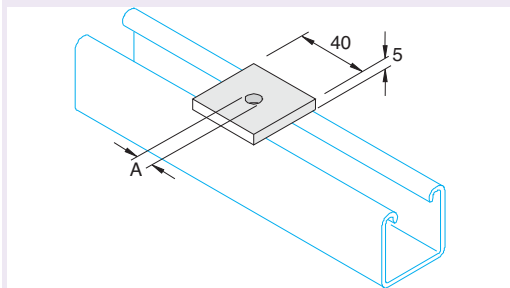
Square Plate Washer
